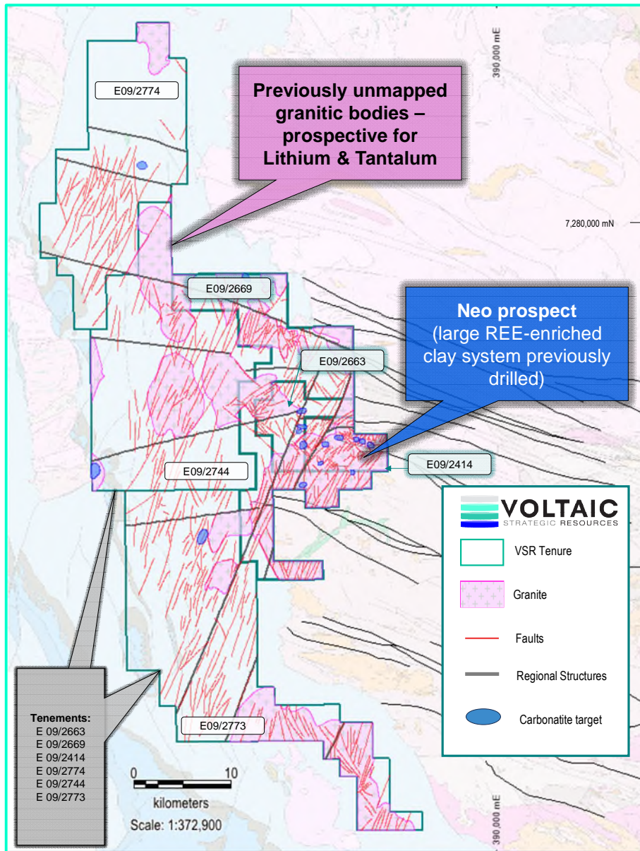
Figure 17. Paddys Well project with interpreted carbonatite targets and regional geology
