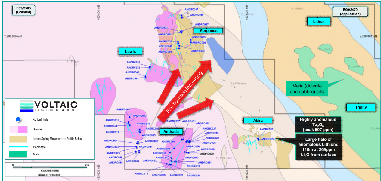
Figure 7. Drill map plan of Andrada, Lewis, Morpheus & Akira prospects at Ti Tree (South)
