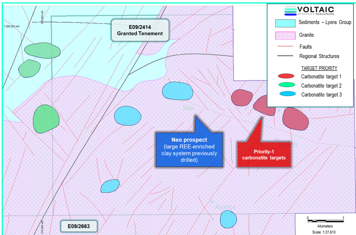
Figure 16. Carbonatite targets in close proximity to recent drill target area within granted tenement E09/2414.
