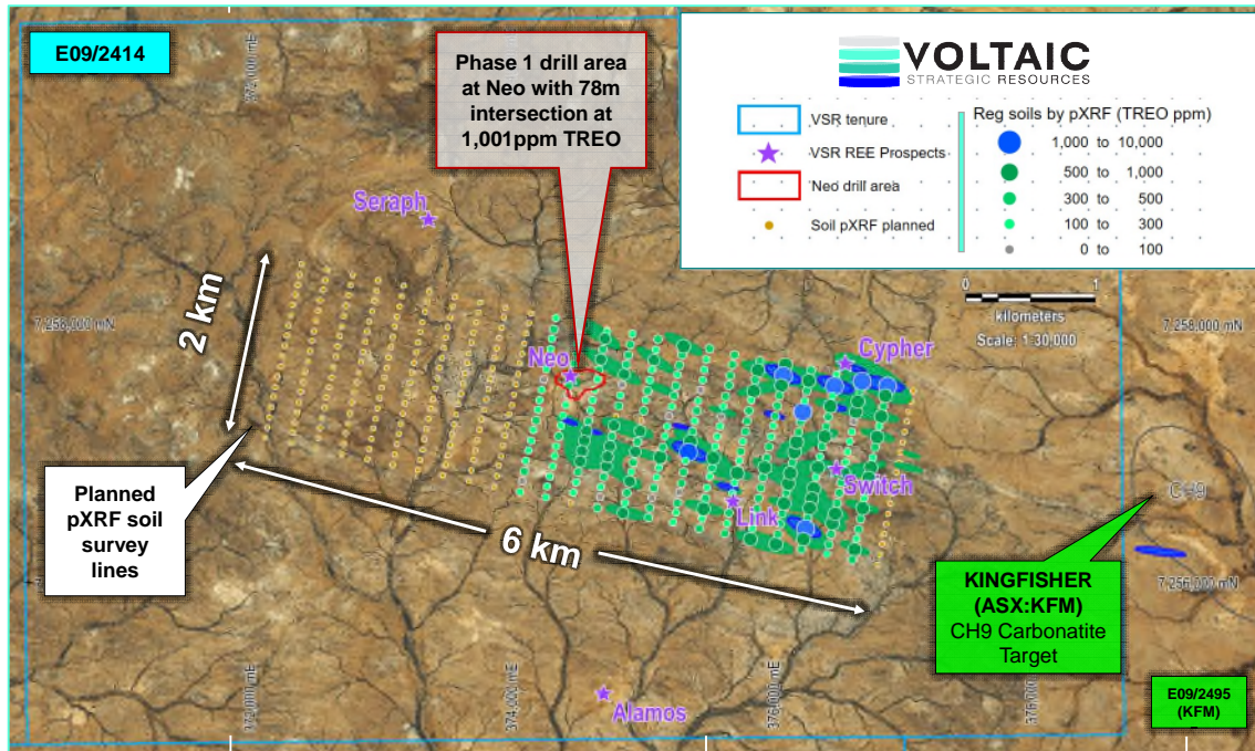
Figure 14. TREO contours at the Neo prospect within regional 6 x 2km anomalous area.
