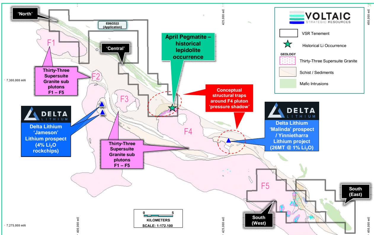
Figure 10. Ti Tree project map with granitic sub-plutons of the Thirty Three Supersuite shown (F1-F5)
