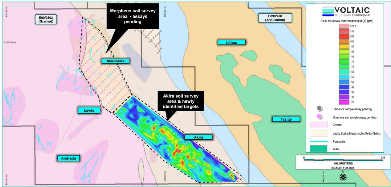
Figure 9. Akira prospect regional soil sampling survey – lithium in soil anomaly
