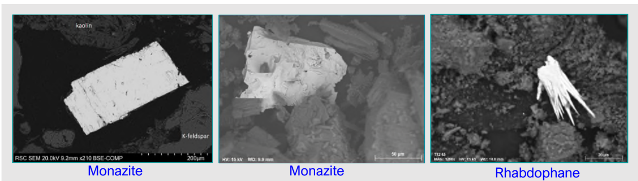
Figure 13. Monazite & rhabdophane (REE phosphate) crystals identified from SEM analysis of REE-enriched clay samples from historical drillhole GAD0004
