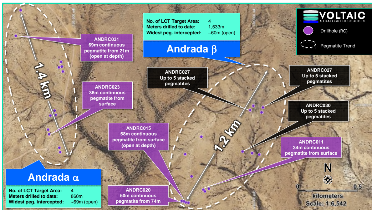
Figure 6. Drilling map showing holes completed at Andrada prospect with identified pegmatite trends.
