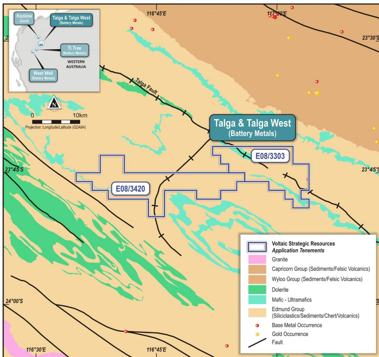
Figure 12 – Local geological setting of the Gascoyne Battery Metals Projects (Talga & Talga West).
